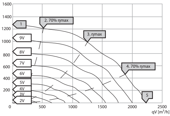
psf [Pa] KCF-N 225 EC 30
