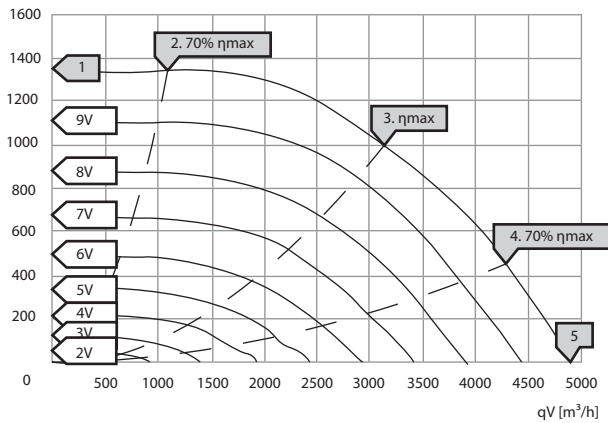
psf [Pa] KCF-N 315 EC 21
