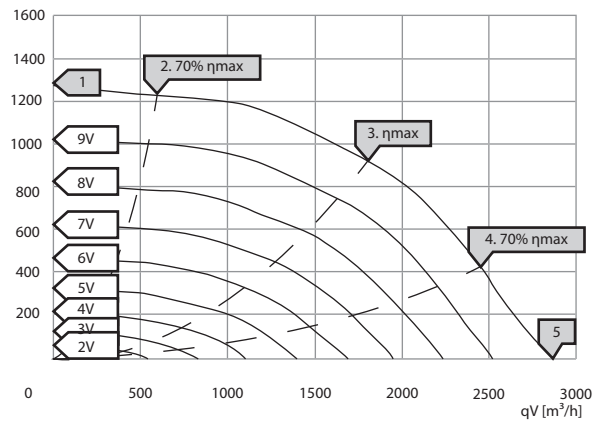
psf [Pa] KCF-N 250 EC 30
