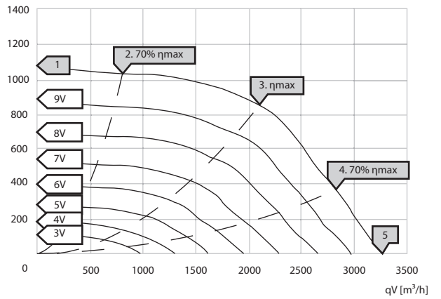
psf [Pa] KCF-N 280 EC 30
