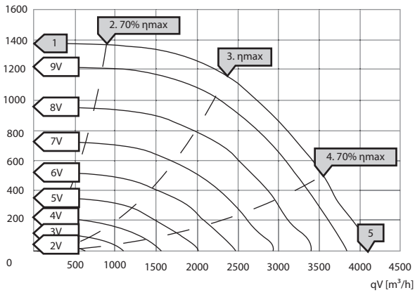
psf [Pa] KCF-N 280 EC 20
