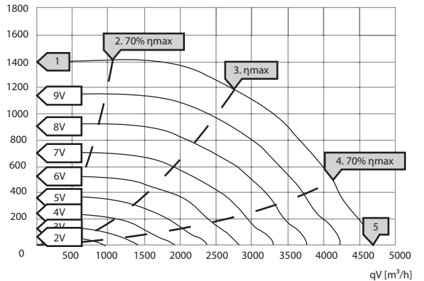
psf [Pa] KCF-N 315 EC 30
