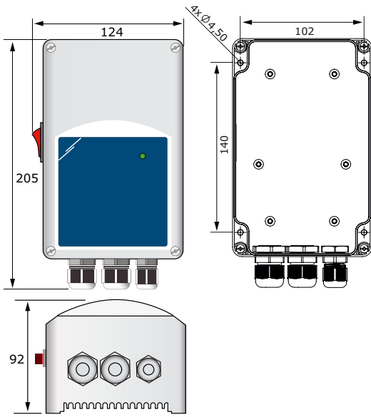
Fig. 1 Mounting dimensions
