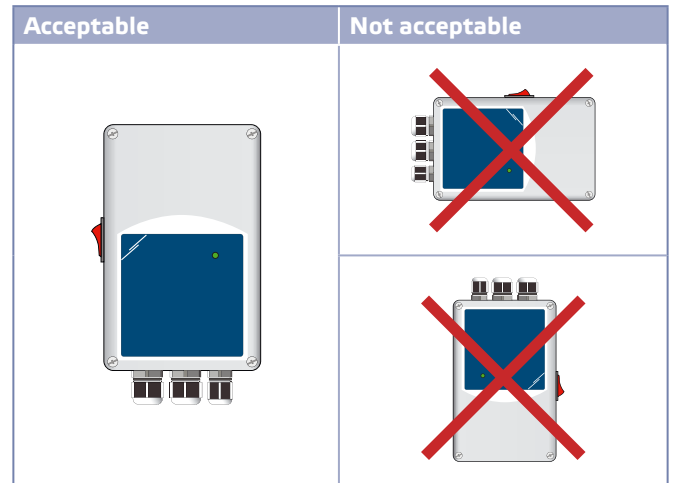
Fig. 2 Mounting position
