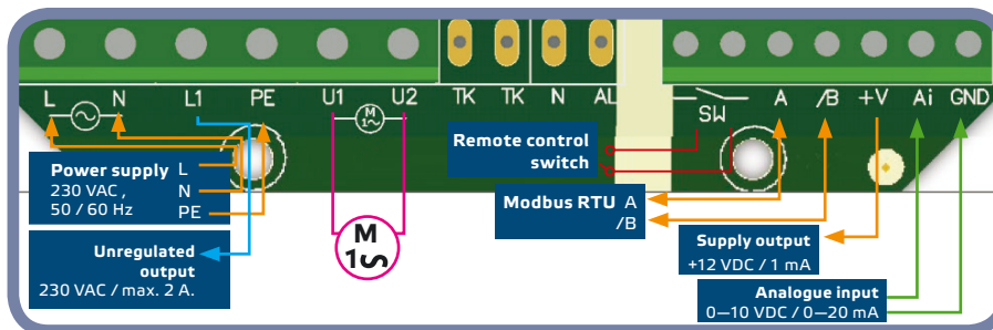
Fig. 3 Wiring and connections
