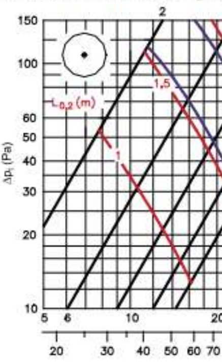
KTS-100-C without sector plate
