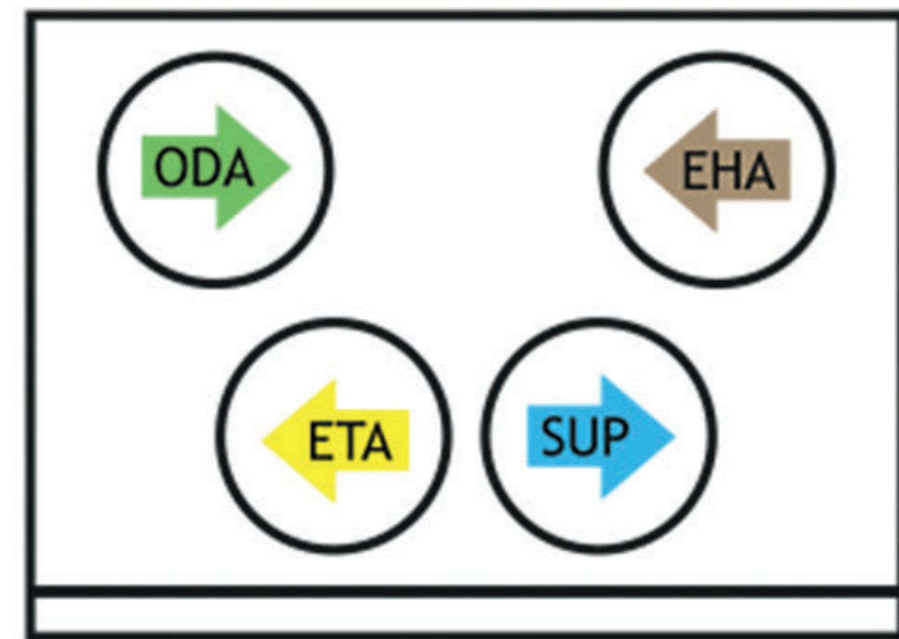
View from inspection side
