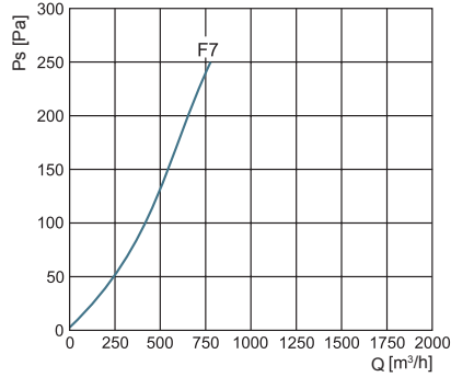
FLF-B 400
