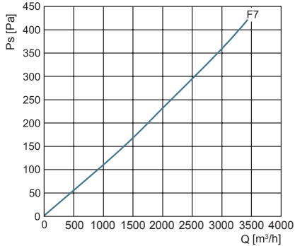
FLF-B 355
