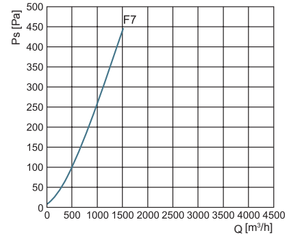
FLF-B 315
