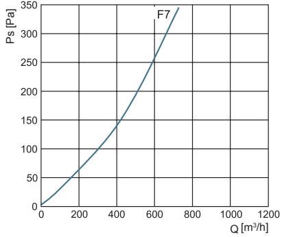
FLF-B 355
