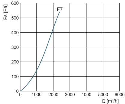
FLF-B 400
