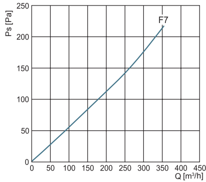
FLF-B 250
