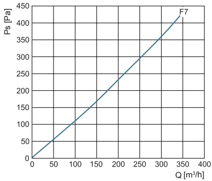
FLF-B 200
